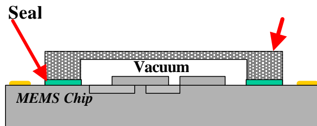
Figure 1 – Zero-Level Hermetic Package
